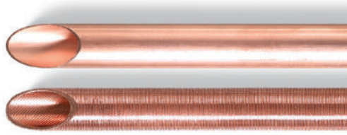
2012~2016 SS316L Tube
